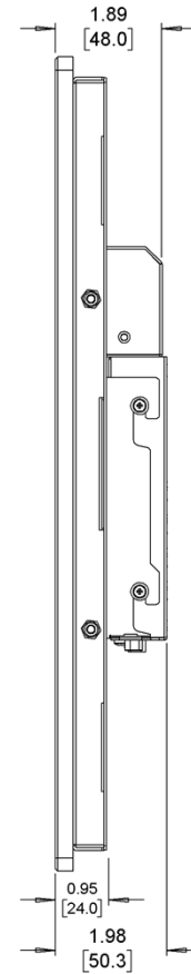
SIDE VIEW
