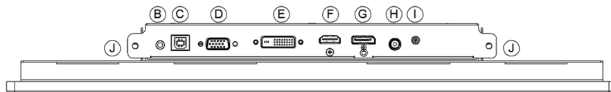
BOTTOM VIEW
